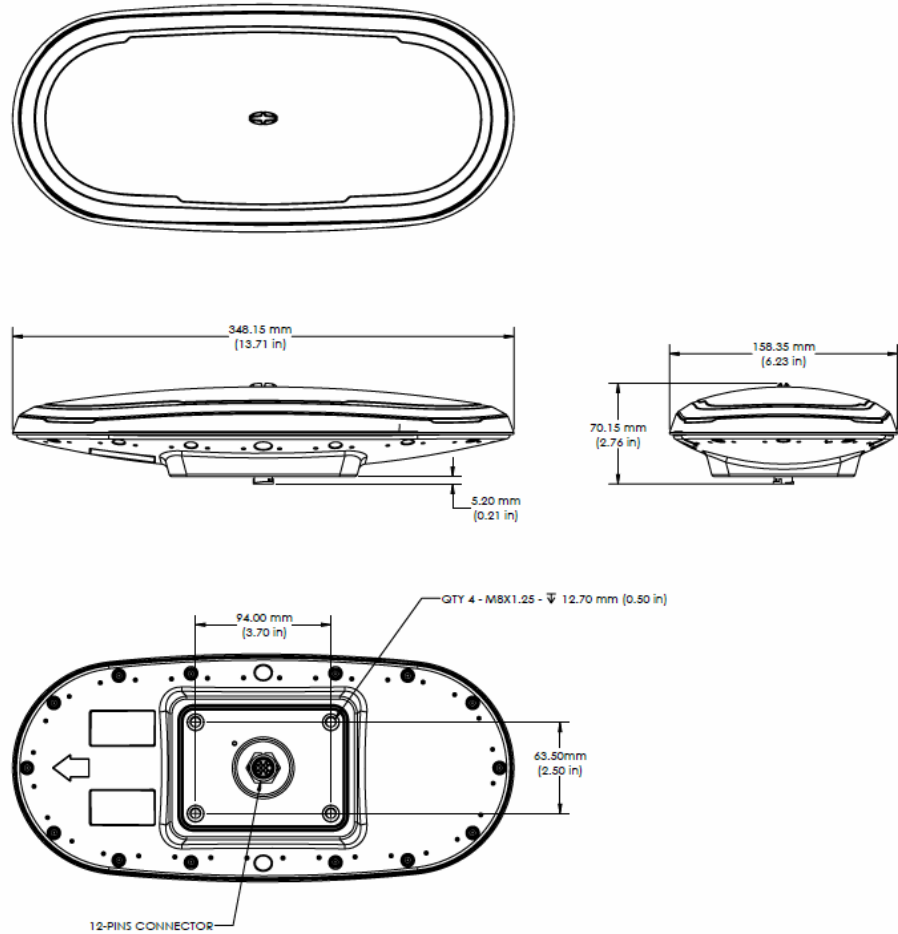
Figure 2-5: V200s dimensions
